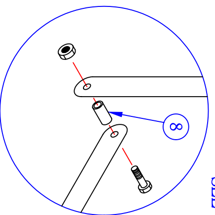
VIEW 'B'
